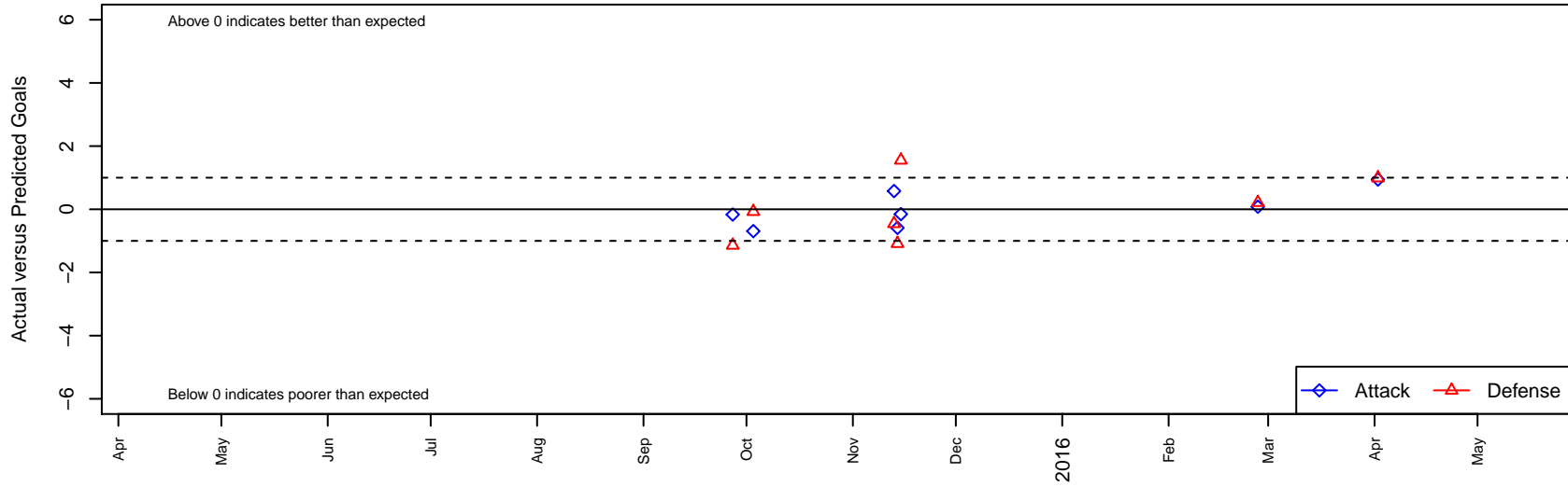
Sereno Southeast Chelsea 98 White G97 Dots are actual minus expected GF (blue circles) and GA (red triangles). Blue line is smoothed change in attack strength. Red is smoothed change in defense strength.
